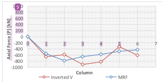
FIGURE 6. Comparison of Axial Force Distribution of MRF and CBF - Inverted V (Part.1)
