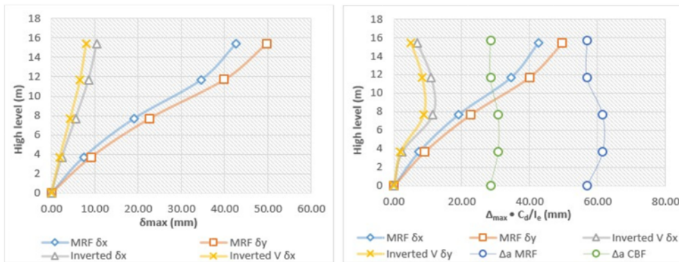
FIGURE 9. Comparison Story Displacement
