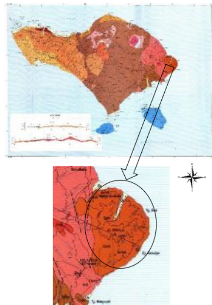
Fig. 3. Regional Geology.
