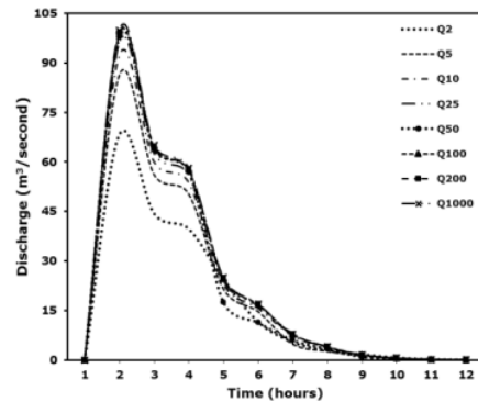
Fig. 9. Nakayasu synthetic unit hydrograph
