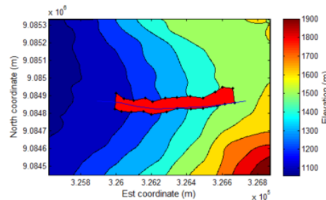
Fig. 7. Results of the DFLOWZ analysis
