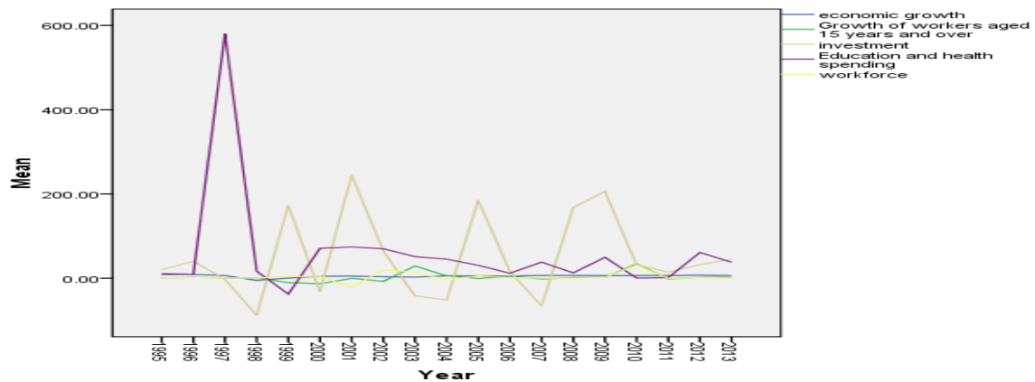
Figure 3: Descriptive Analysis 1995-2013 (%)
