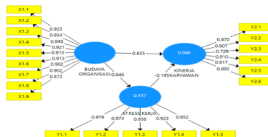
Figure 2. Outer Loading and Path Analysis Estimated Results
