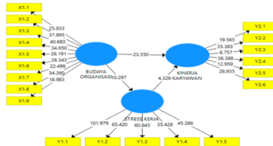
Figure 3. Bootstrapping (Test Statistics)
