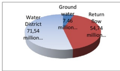
Figure 1. Water Pontential in Saba Watershed
